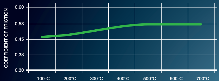
FRICTION vs. TEMPERATURE RSH 3
